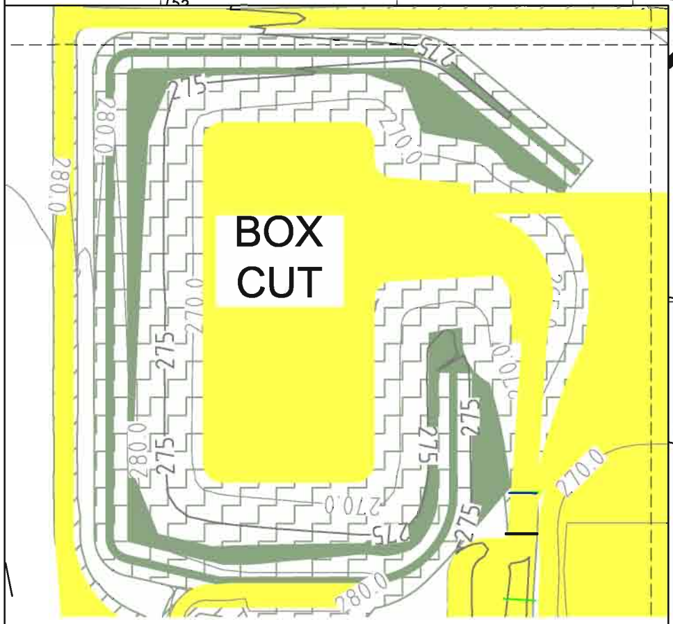
BOX CUT DETAIL
